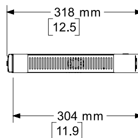
RIGHT VIEW
